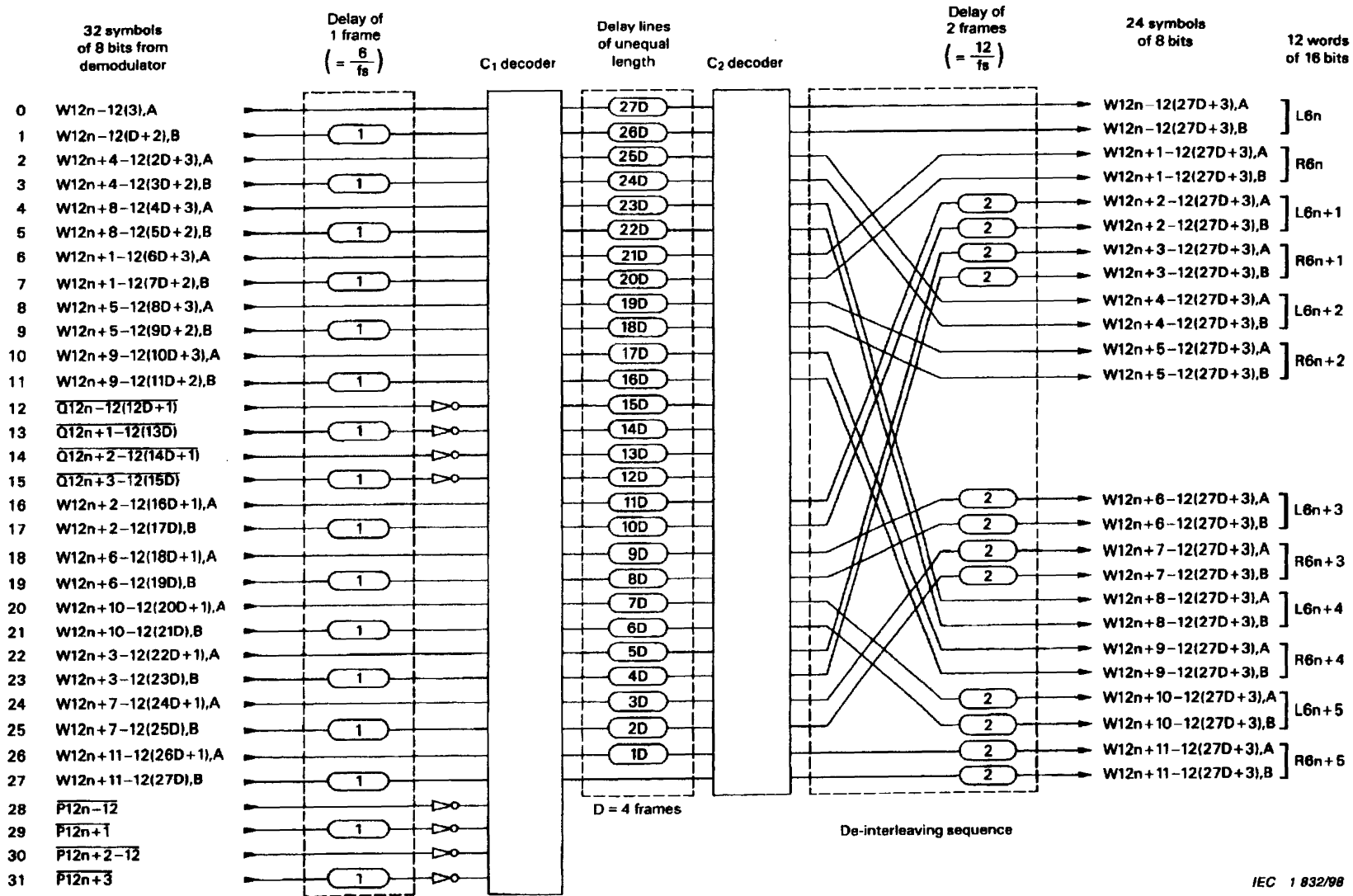
Figure 13 – CIRC decoder
