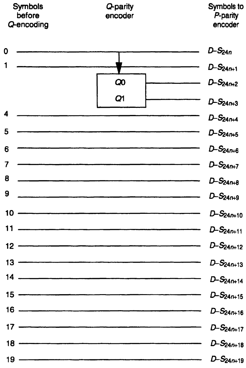
Figure 23 – Q-parity encoder
