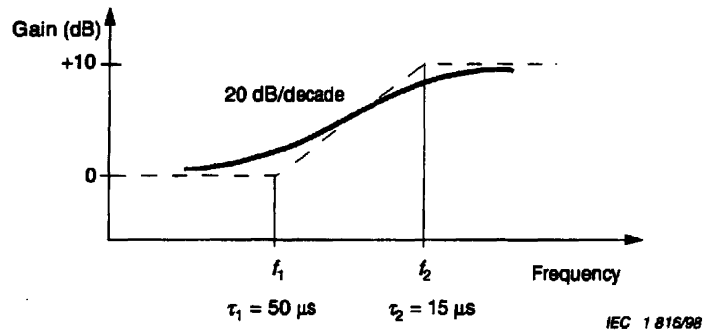
Figure 1 - Pre-emphasis characteristic
