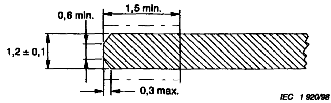
Figure 2d – Edge shape of the disc (8 cm-CD)
