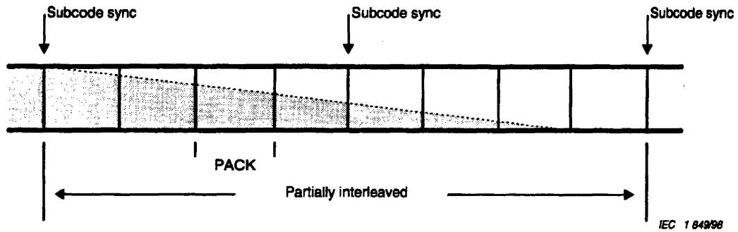
Figure 30 – Example of partial interleaving of PACKs
