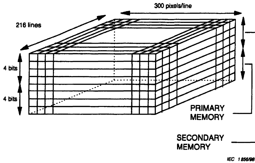
Figure F.1b - One memory plane of 256 colours
