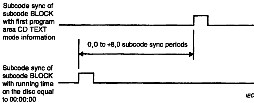
Figure 31 – Maximum allowed mode transition skew
