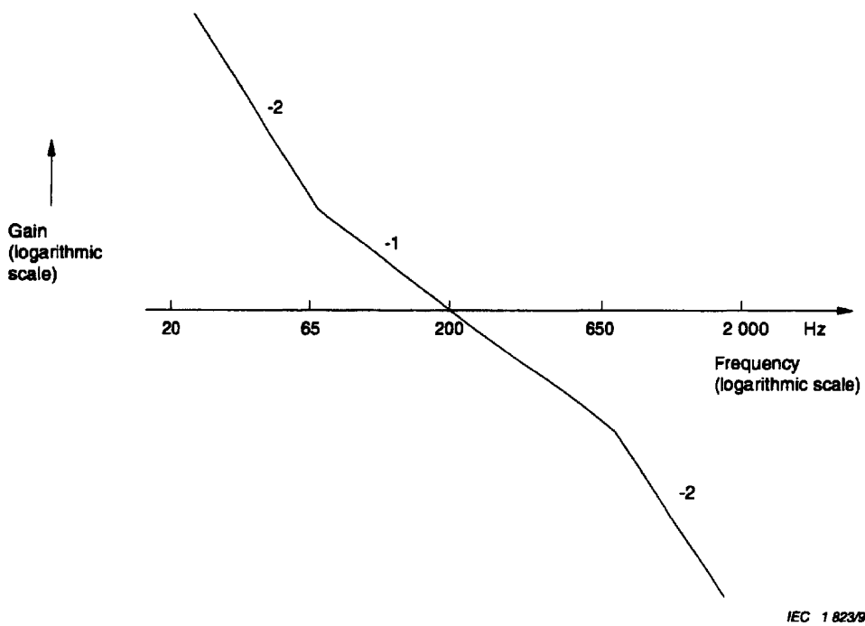
Schematic representation of the open-loop transfer function for tracking measurements.
