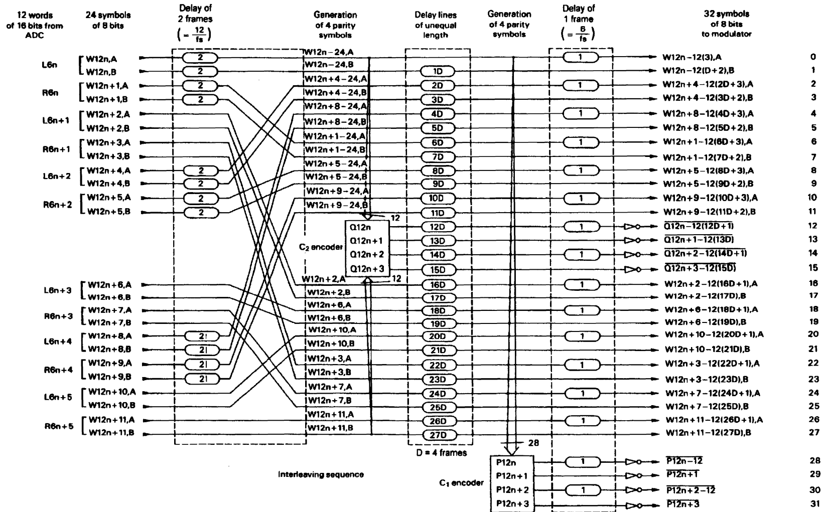
Figure 12 – CIRC encoder
