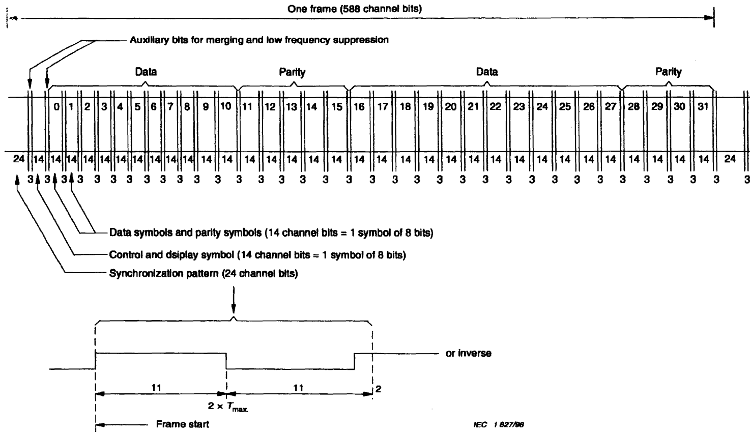
Figure 8 – Frame format
