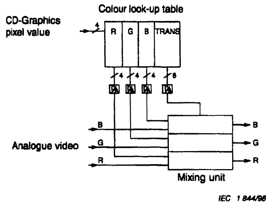
Figure 25 – Block diagram of a video/graphics mixing unit
