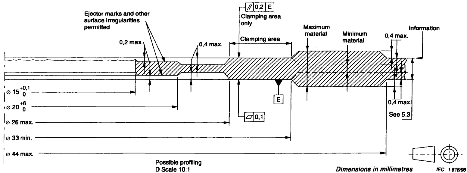
Figure 2b – Dimensions of the disc
